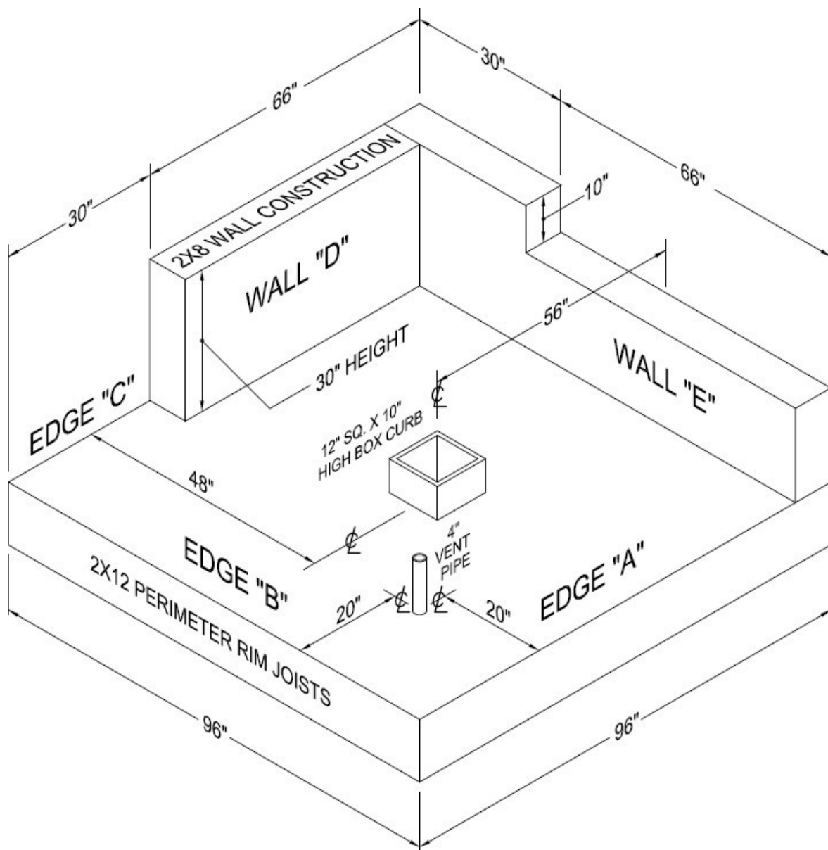
Mockup Design for SkillsUSA Roofing Demo (Thermoplastic)
